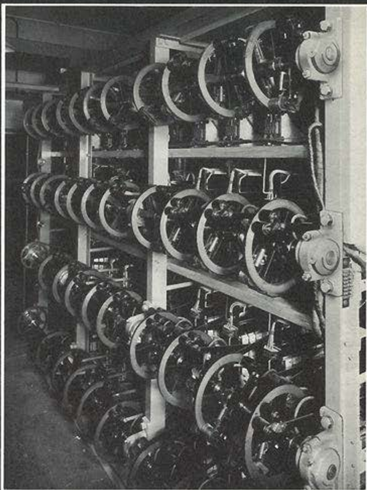
▶ Mansell magnetic clutches and Sunset dimmers of the Thirties.
