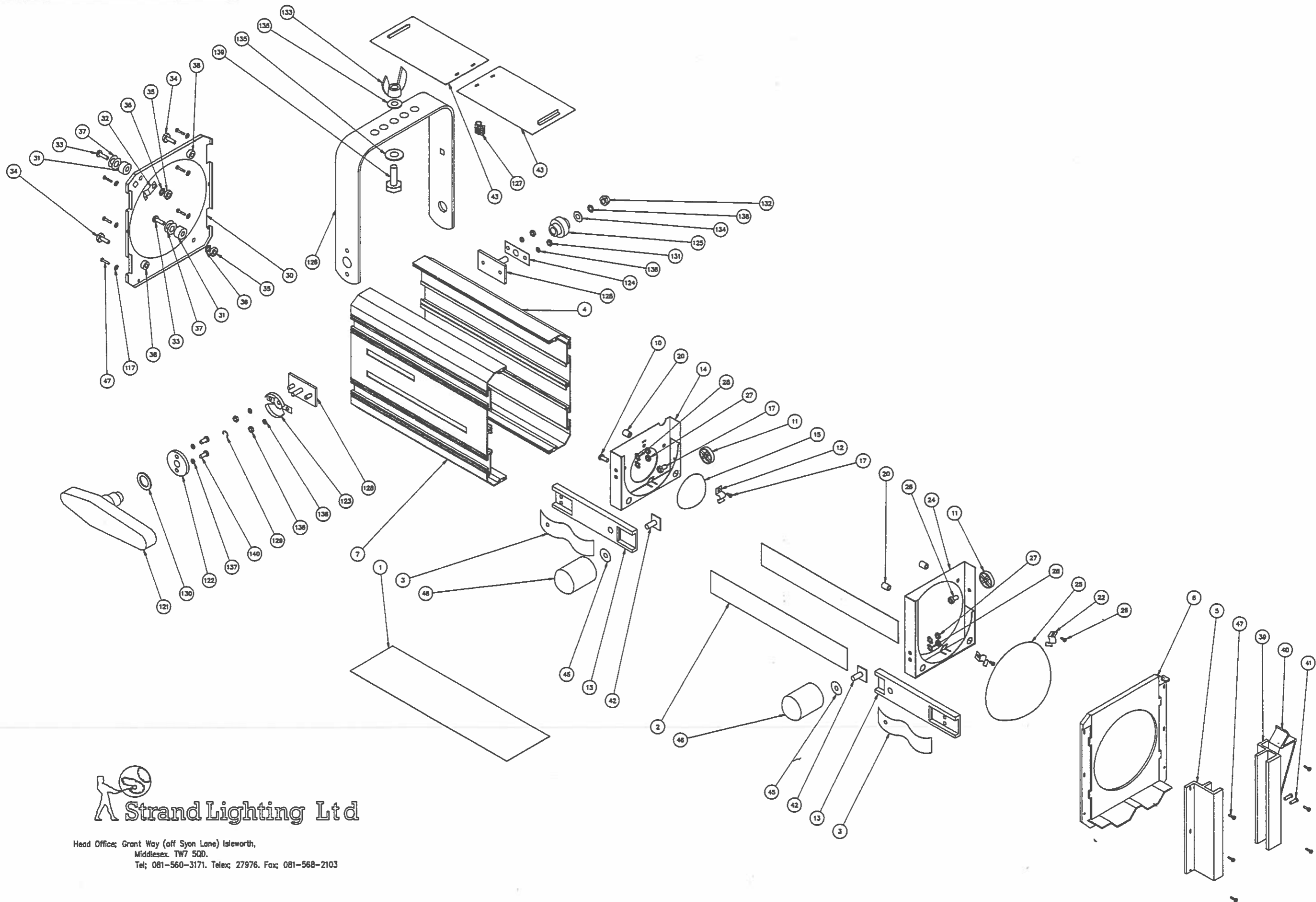
CANTATA 18/32 LENS ASSEMBLY & MOUNTING FORK
