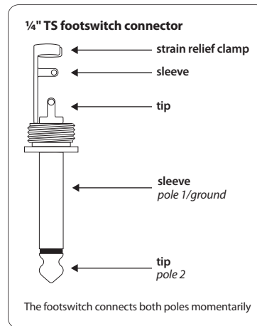
Fig. 9.3: Footswitch connector
