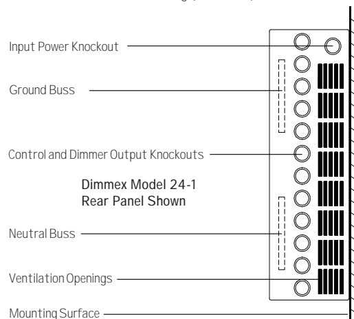
Wall Mounting (Side View)
