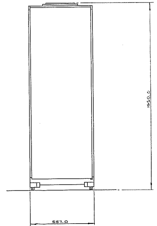
EQUIPMENT RACK FOR SYSTEMS UP TO 640 WAYS.
