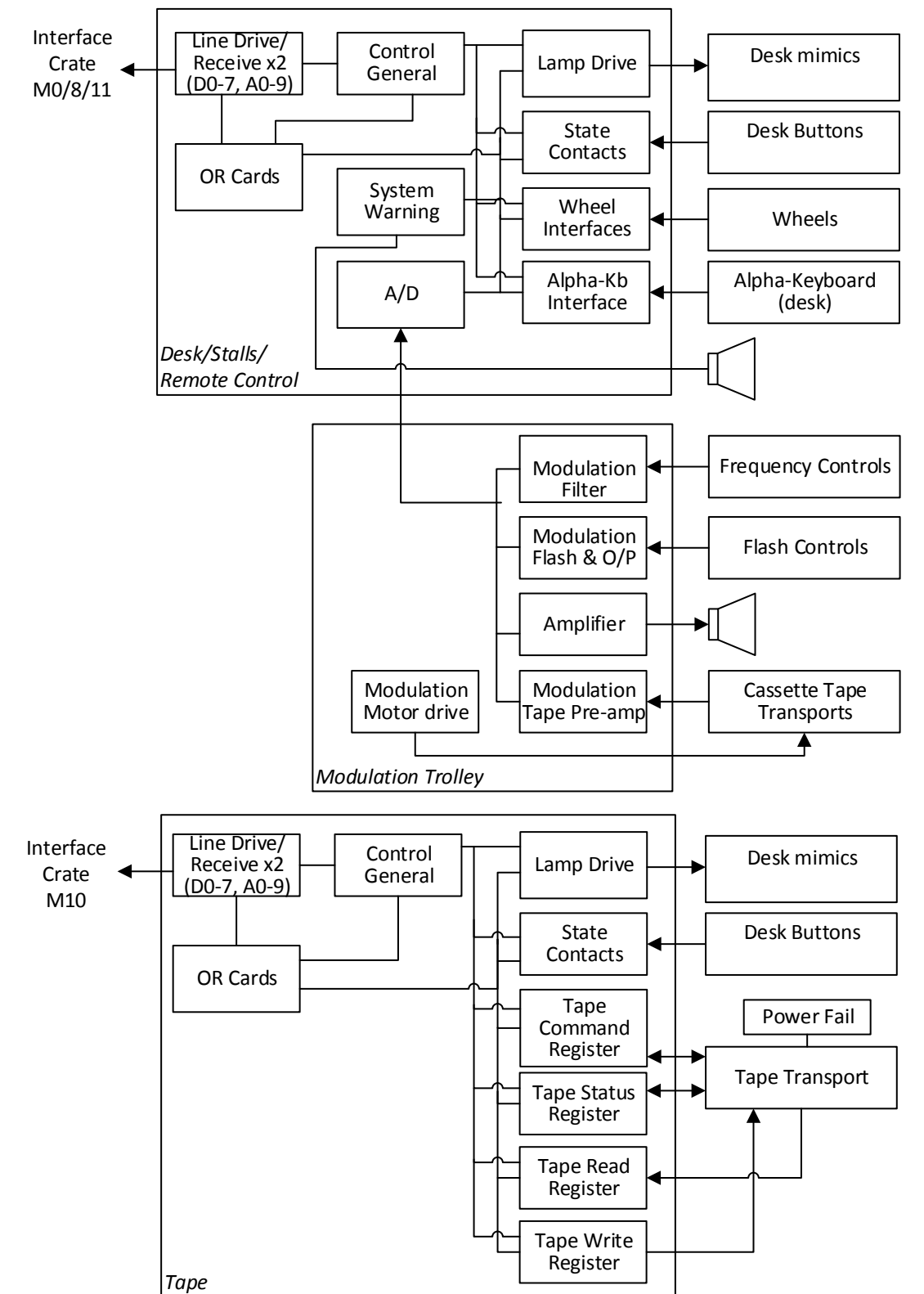
Lightboard, TCS Interconnection Diagram Rev 1.0 David Bertenshaw, 29-sept-2020
