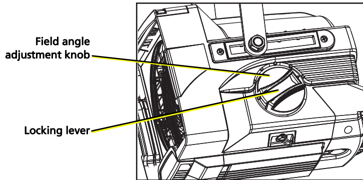
Figure 4: Field angle adjustment knob and locking lever
