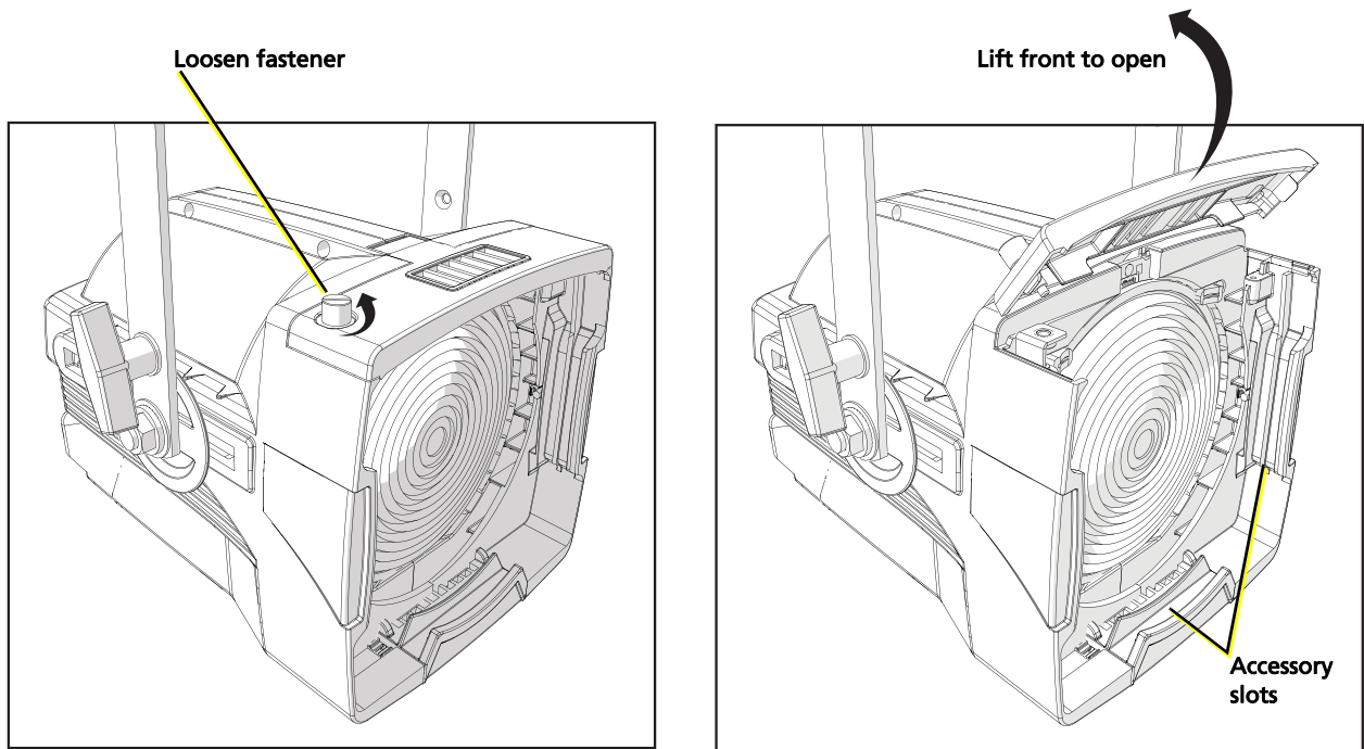
Figure 8: Accessory holder door releases
