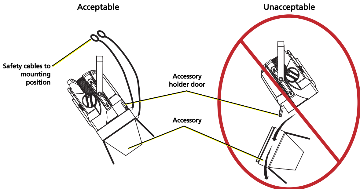
Figure 7: Fixture with accessories
