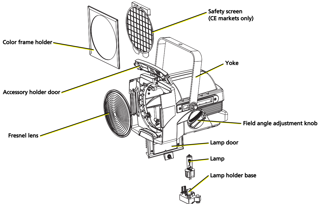
Figure 1: Source Four Fresnel fixture components
