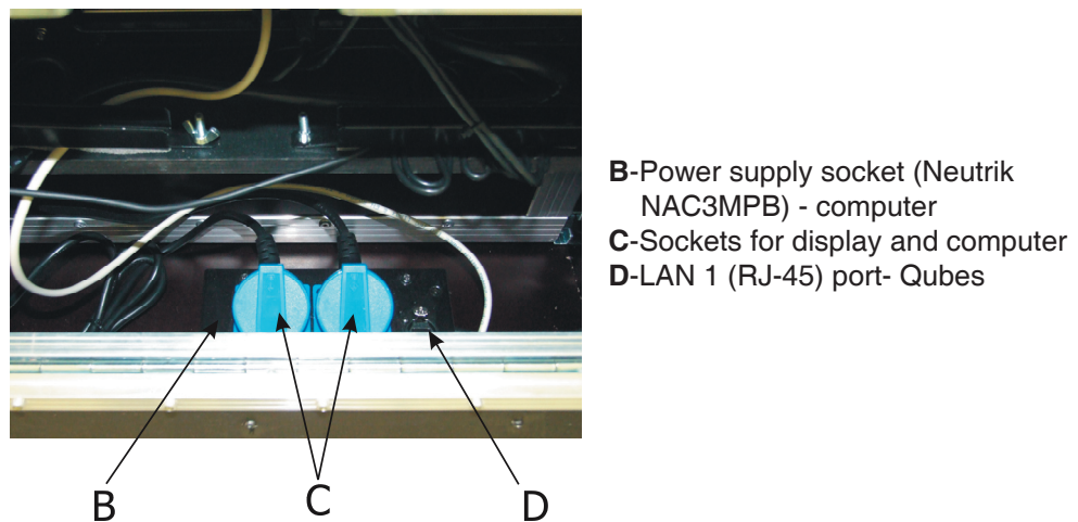
Detail of the connection block
