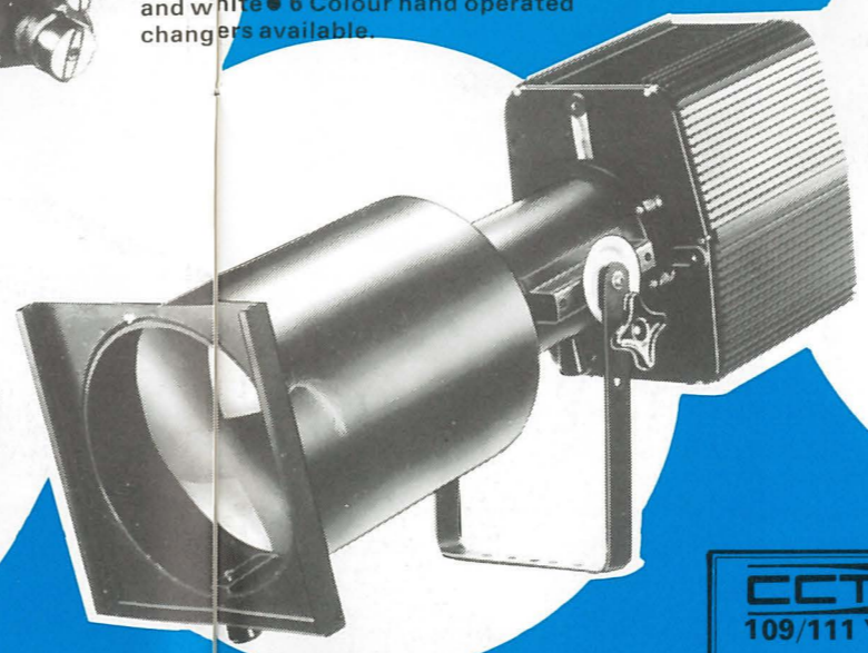
SILHOUETTE 1000W & 2000W The standard against which all profile spotlights are measured. Interchangeable lens tubes—Variable lens combinations 10°-15°-25°-30°-40°
