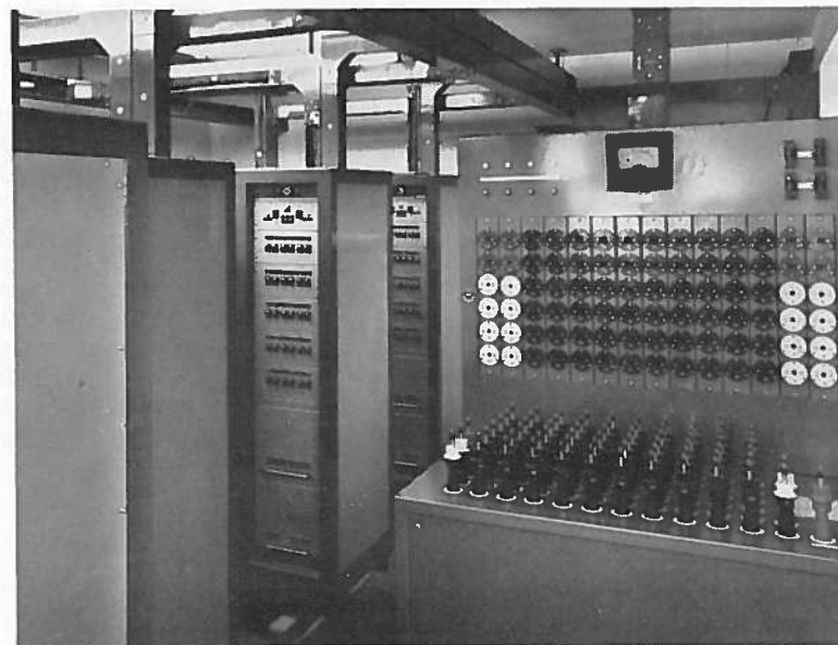
Fig. 3. Part of the dimmer room showing patch panel in foreground and Thyristor (System CRD) racks on the left.
