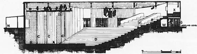
SECTION ON CENTERLINE ANTA-WASHINGTON SQUARE THEATER FOR THE LINCOLN CENTER REPERTORY COMPANY
