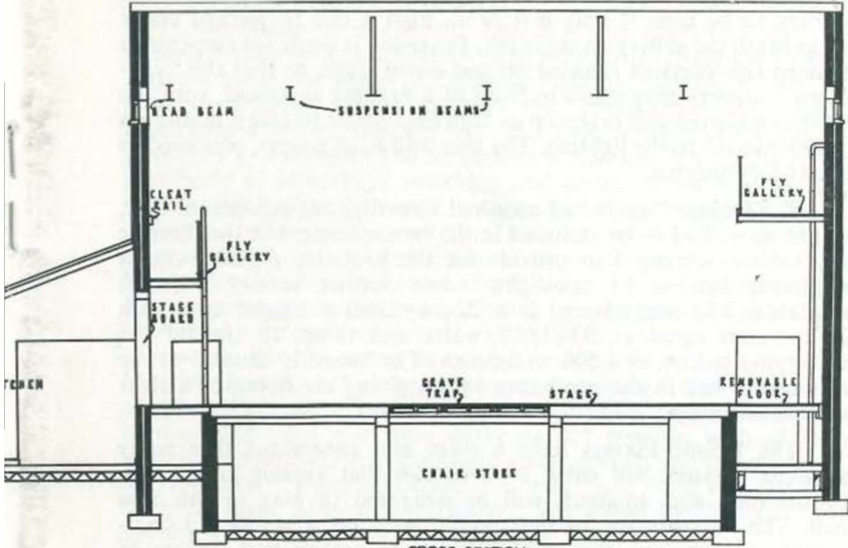
CROSS SECTION
