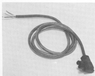
35 000 00 : 1.5m Power Cable, wire-end 35 002 01 : 1.5m Power Cable, 15A 3-pin 35 001 06 : 1.5m Power Cable, Schuko
