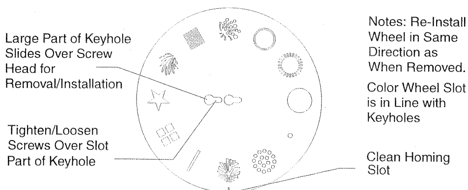
Figure 8.3. Wheel Mounting Slots and Orientation
