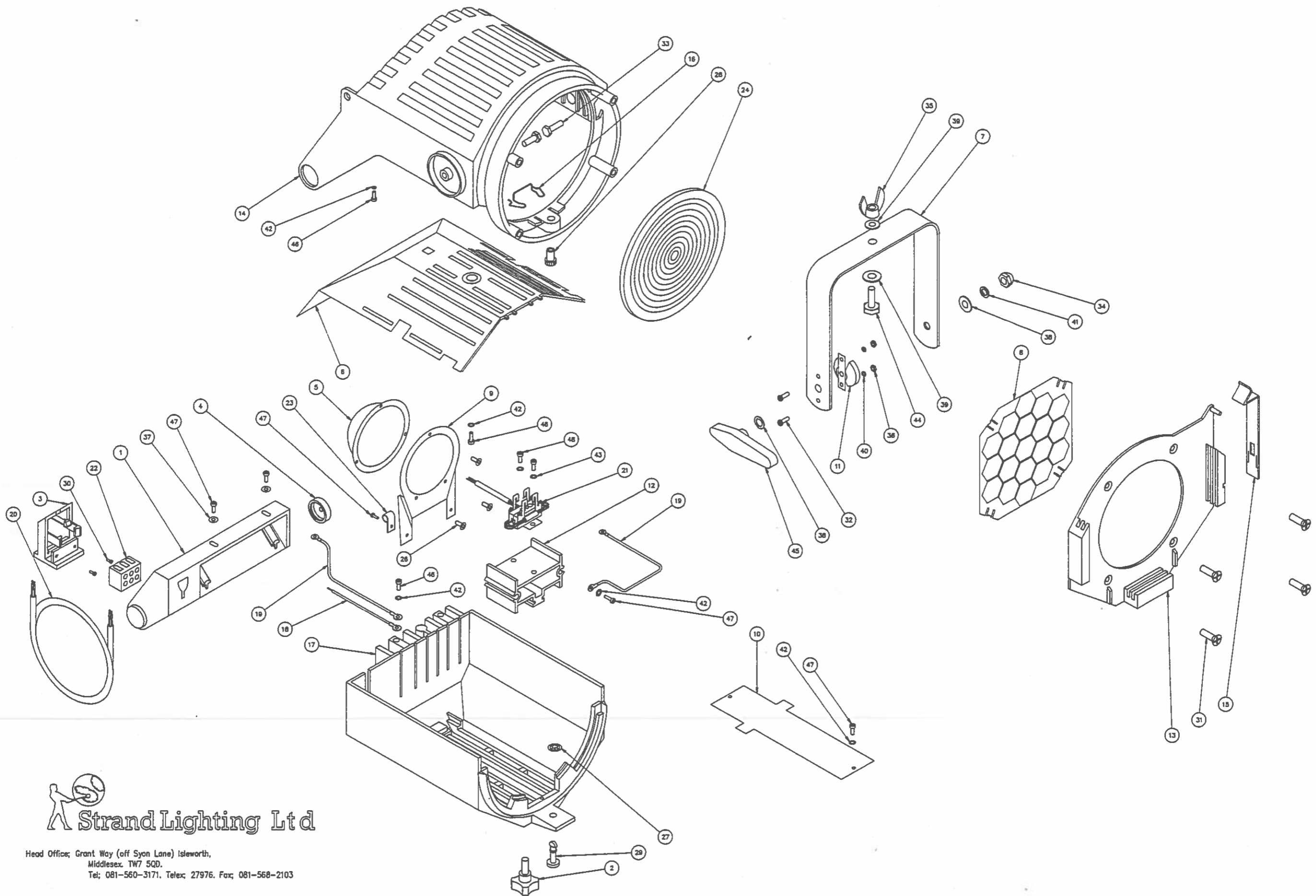
QUARTET "F" LAMP ASSEMBLY
