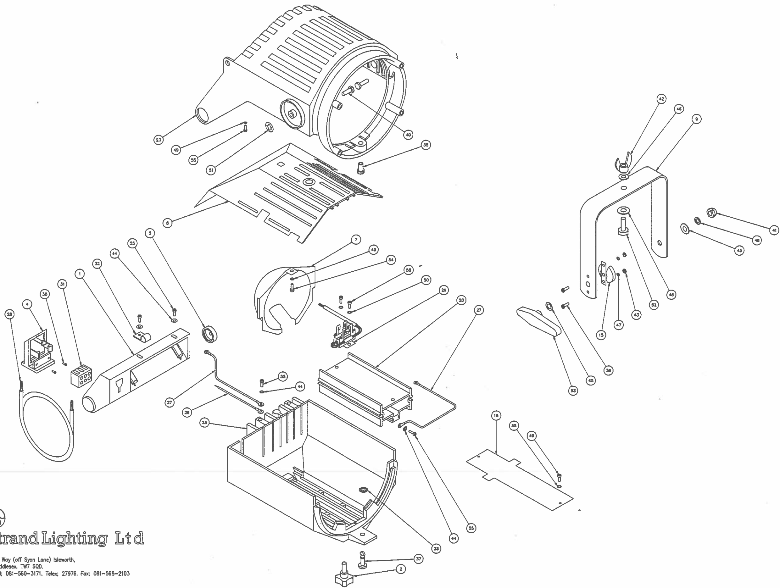
QUARTET 22/40 LAMP ASSEMBLY
