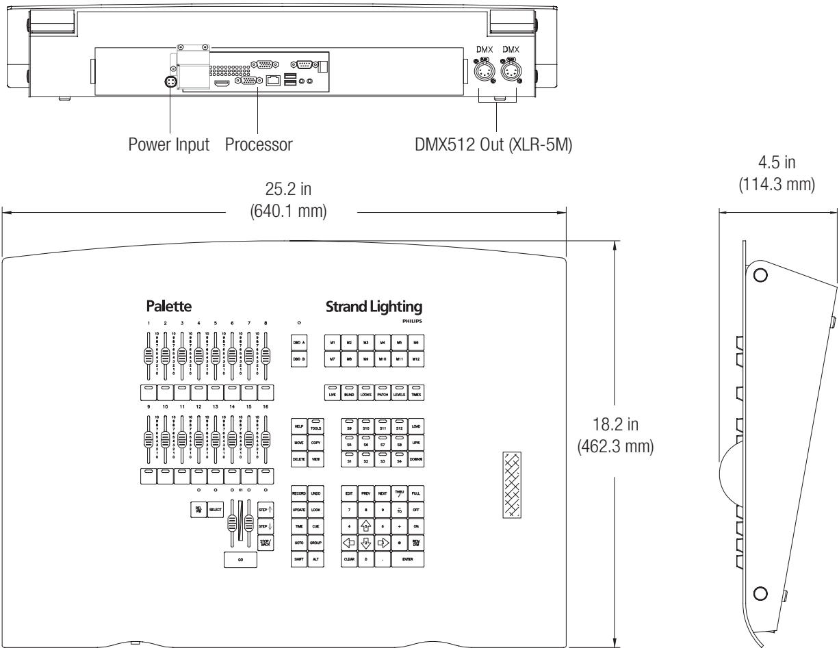
92800 Basic Palette II Memory Console with 250 Channels, 16 Submasters
