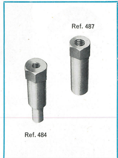
Ref. 484 Spigot Adaptor for \frac{3}{8} -in. bolt. For Patt 23, 45, 60, 123, 137, 202, 223, 263, 264. Weight \frac{1}{4} lb. (0.35 kilos). Ref. 487 Spigot Adaptor for \frac{1}{2} -in. bolt. For Patt 49, 149, 243, 252, 253. Weight \frac{1}{4} lb. (0.35 kilos). Supplied with Patt. 265, 293.
