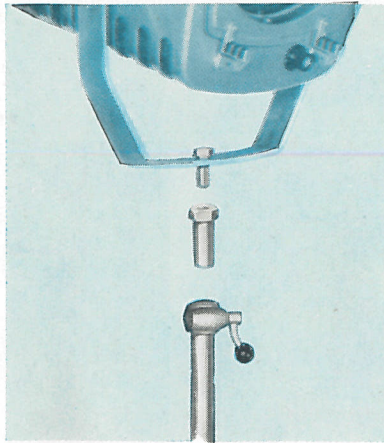
Ref. 484 Spigot Adaptor for \frac{3}{8} -in. bolt. For Patt 23, 45, 60, 123, 137, 202, 223, 263, 264. Weight \frac{1}{4} lb. (0.35 kilos). Ref. 487 Spigot Adaptor for \frac{1}{2} -in. bolt. For Patt 49, 149, 243, 252, 253. Weight \frac{1}{4} lb. (0.35 kilos). Supplied with Patt. 265, 293.
