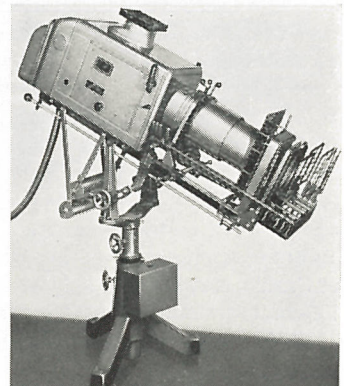
2000-watt Patt. 511 Xenon Arc
