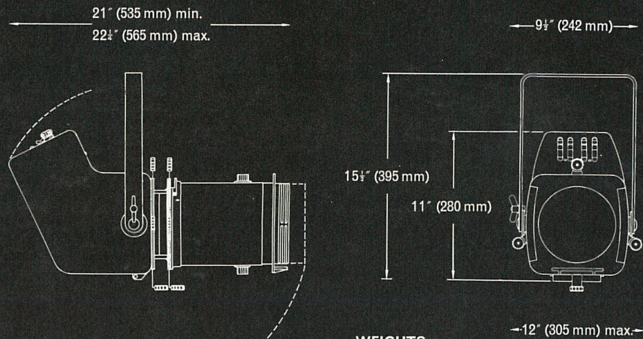
SCALE 1:10
